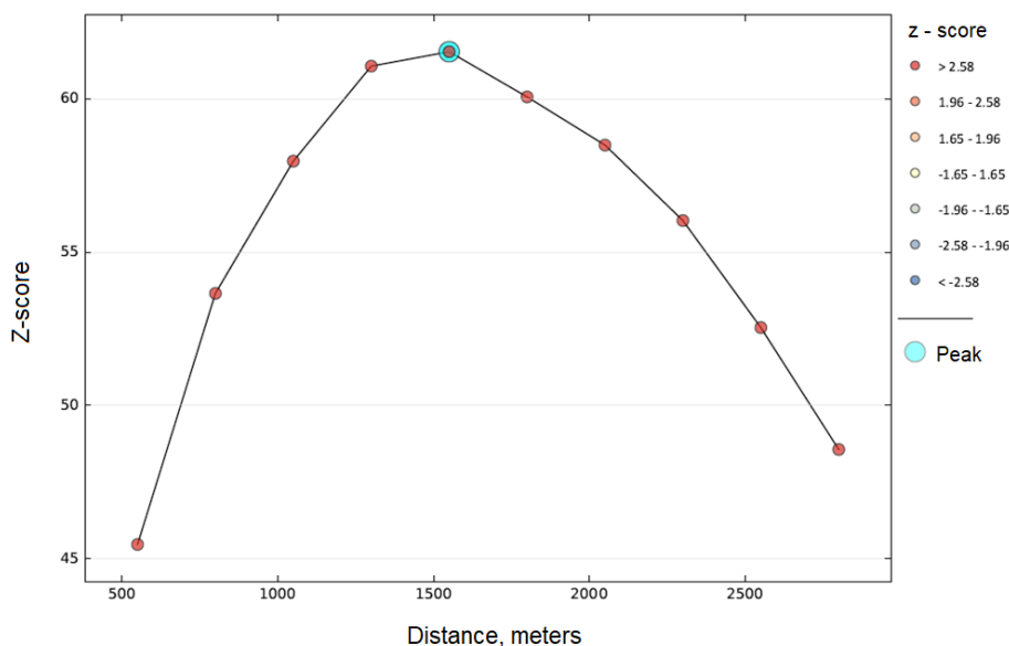
Fig. 2. Graphical interpretation of the minimum distance of the neighborhood search neighborhood between the values of the content of acid-soluble copper in the soil
