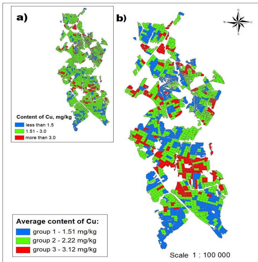
Fig. 1. Spatial localization of identified groups of acid-soluble copper content clusters within the land use of the RUE «Educational Experimental Farm of BSAA»
